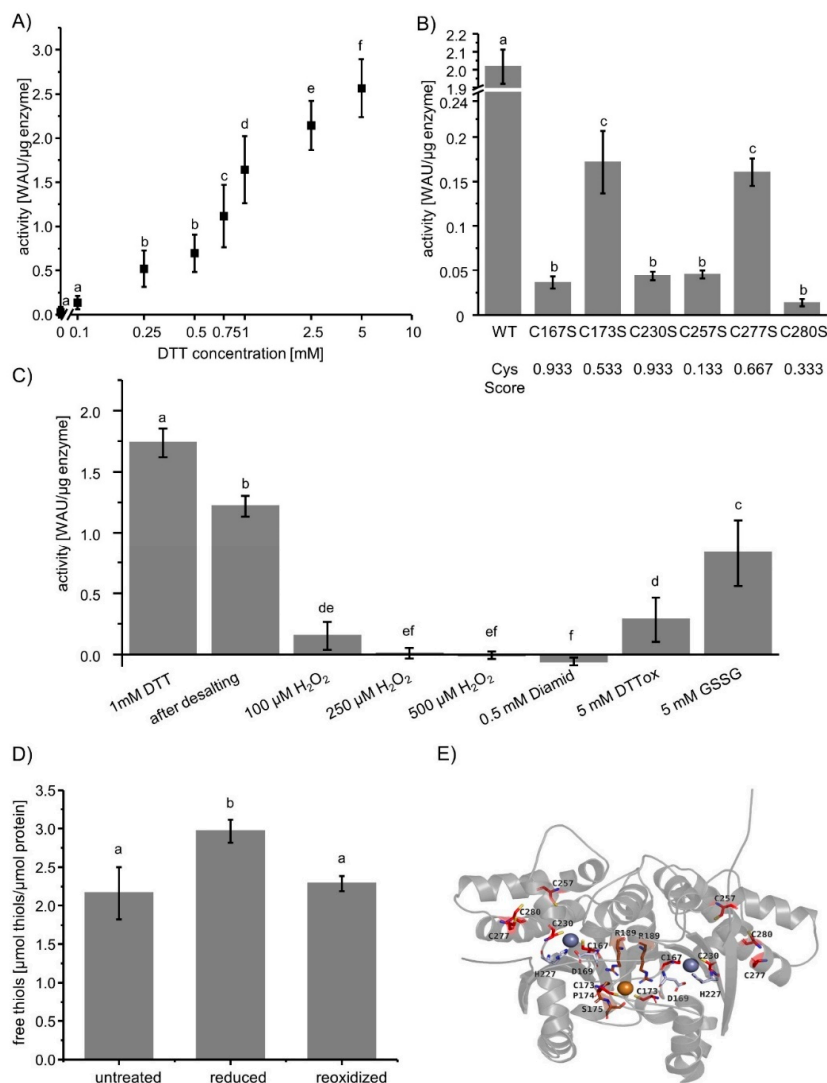
Figure 1. Redox-dependent activity of wildtype βCA1 and its Cys → Ser variants. (A) βCA1 activity after treatment with increasing DTT concentrations for 30 min at room temperature. Letters a–f indicate significant differences at p \leq 0.05 , as calculated using one-way ANOVA with post hoc Tukey HSD test. Data are means \pm SD of n \geq 13 from two independent protein purifications. (B) Activity of βCA1 and its Cys variants after preincubation with 1 mM DTT for 30 min at room temperature. Data are means of n \geq 6 \pm SD from two independent protein purifications. Significant differences at p \leq 0.05 were calculated using one-way ANOVA with post hoc Tukey HSD and are represented by letters a–c. Furthermore, the Cys-Score >0.5 indicates whether the Cys residues are conserved in plant βCA. (C) Activity of βCA1 after reduction with 1mM DTT, desalting, and re-oxidation with different amounts of H 2 O 2 , diamide, DTT ox , and oxidized glutathione. Data are means \pm SD of n \geq 6 . Letters a–f indicate significance of difference calculated with one-way ANOVA and post hoc Tukey HSD. (D) Quantification of thiols of untreated, or reduced (1 mM DTT) and desalted βCA1 either labeled directly or after oxidation with 100 μM H 2 O 2 . Thiols were quantified using Ellman’s reagent. Data represent means \pm SD of n \geq 4 from two independent protein purifications. Significance of difference was calculated using one-way ANOVA and post hoc Tukey HSD and are represented by letters a and b. (E) Structure of the homodimer of βCA1 based on the x-ray structure of CA of Pisum sativum (pdb: 1ekj). Cys are marked in red, zinc binding amino acids, besides C167 and C230, are marked in gray, and copper binding amino acids, besides C173, are marked in brown. The zinc and copper ions are shown as spheres in gray and brown, respectively. The homodimer has two active sides where the zinc is bound by C167, D169, H227, and C230 in each subunit. The copper ion is bound by C173, P174, S175, R189 from Chain A and C173 and R189 from Chain B.
