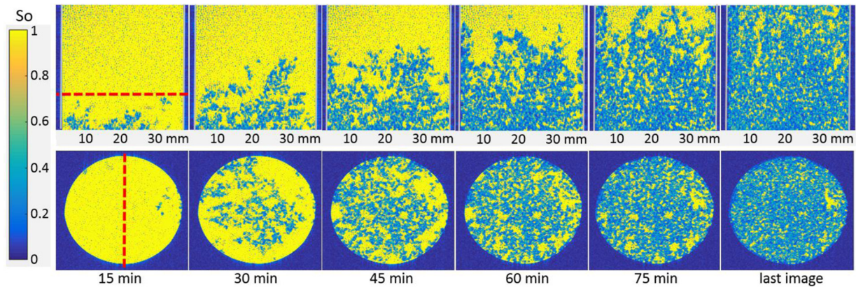
Fig. 4. Consecutive MRI images of the water–oil displacement in the model of polystyrene beads with the injection flow rate of 0.12 mL/min. The oil is yellow and the water is light blue. The acquisition of MRI signal was made each 15 minutes and shown here from the first water appearance in FOV. The dotted line on the first vertical section indicates the position of the horizontal sections (and vice-versa for the horizontal section below).
