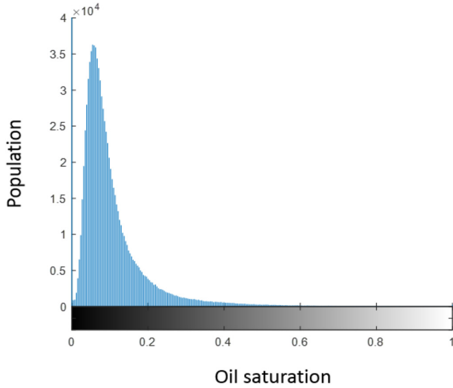
Fig. 10. Histogram of residual oil distribution corresponding to its population in sand beads model ( Q_{inj} 0.12 mL/min).
