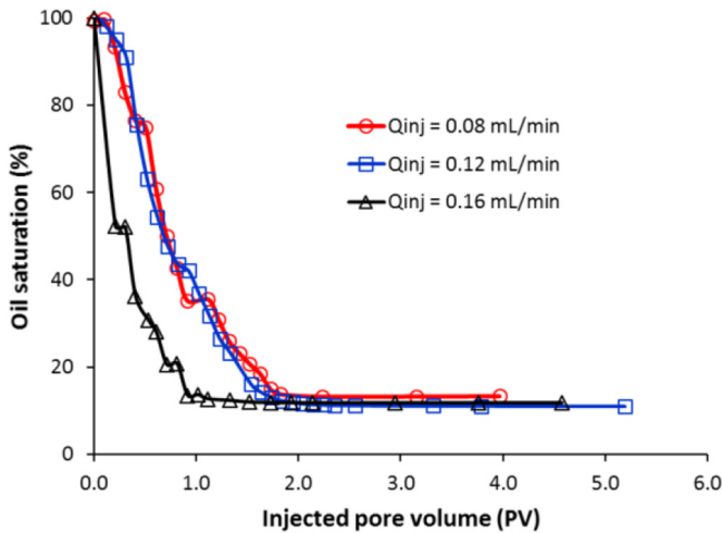
Fig. 11. Averaged oil saturation vs injected PV for the model of packed sand.
