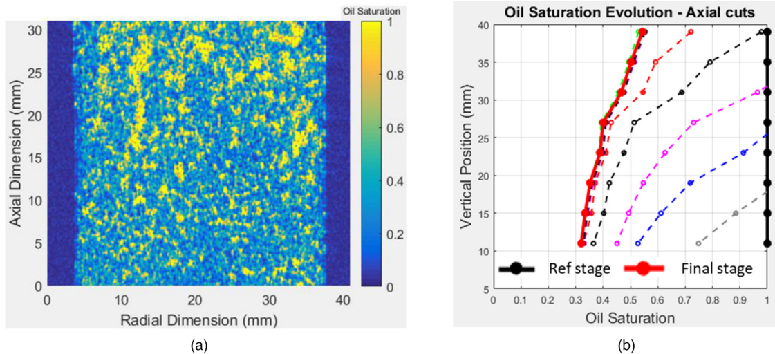
Fig. 5. Residual oil saturation image in a vertical section (a) for the displacement process after the injection of 3.5 PV of the displacing fluid. Time evolution of oil saturation profiles deduced from the 8 axial sections (b).
