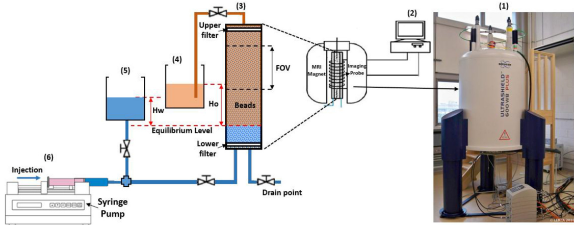
Fig. 1. Experimental setup: (1) 600 MHz NMR system; (2) Computer for data processing; (3) Porous media sample; (4) Oil tank; (5) Water tank; (6) Water injection pump.
