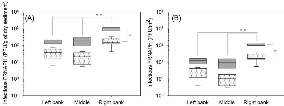
Figure 2. Concentrations of infectious F-specific RNA bacteriophages (FRNAPHs), expressed per gram of dry sediment (A) or per unit area (B), in sediment sampled from the left to the right banks of the river according to hydro-climatological conditions. Dotted box plots represent sediment samples ( n = 9 ) collected during low flow periods (3 sampling points \times 3 campaigns), whereas grey box plots ( n = 3 ) represent samples gathered during the recession phase of a rainfall event (3 sampling points \times 1 campaign). Boxes represent the 25 th and 75 th percentiles, whiskers the 10 th and 90 th percentiles and horizontal line within the box is the median. Stars indicate data significant difference established by a Mann-Whitney Rank test (* P = 0.016 , ** P < 0.001 ).
