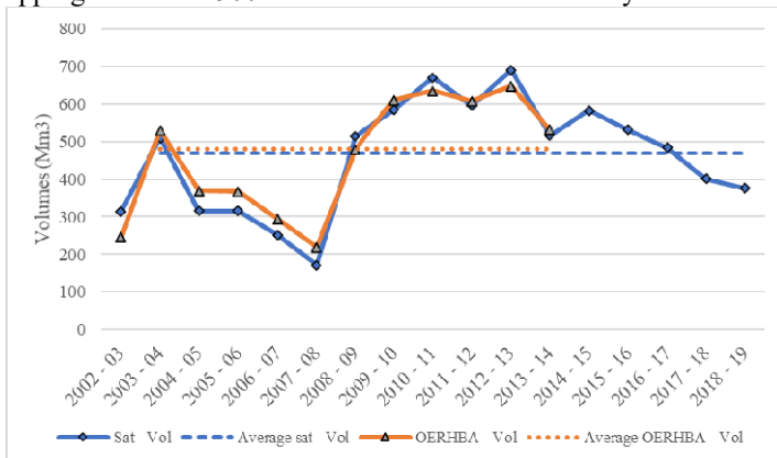
Fig. 11. Maximum annual volume of the AEH's reservoir between 2002-03 and 2018-19.
