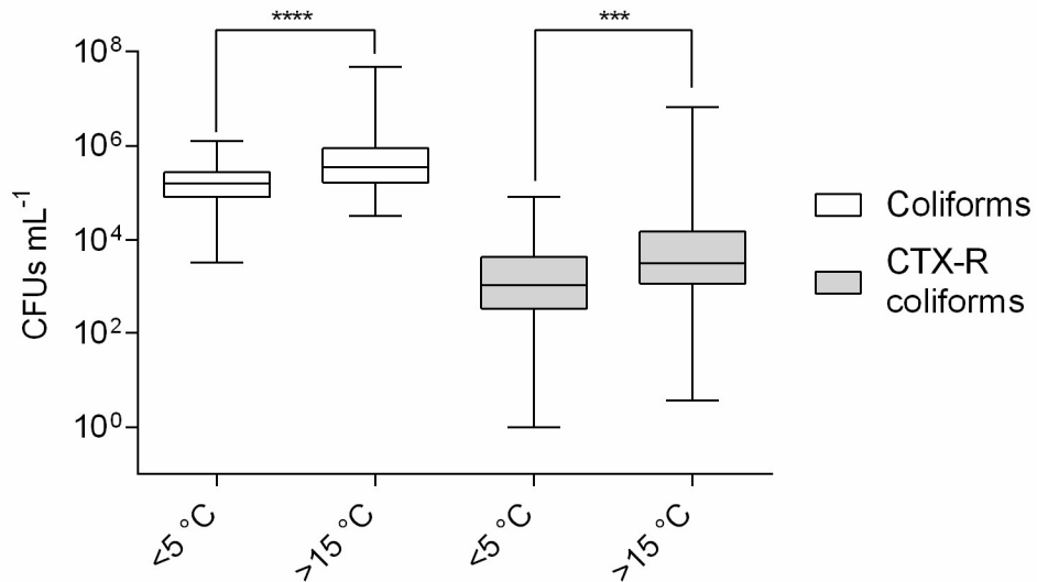
424 Figure 4. Comparison of coliforms and CTX-R coliforms abundance in WWTPs' influent sewage in selected 425 temperature ranks. Asterisks refer to a Mann-Whitney U-test with given p -values <0.0001 (****) and p <0.001 (***).
