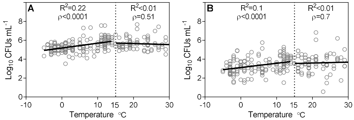
417 Figure 3. Linear regression of log 10 converted coliforms (A) and CTX-R coliforms (B) in WWTP influents as a 418 function of monthly average temperature in the sampled areas. Datasets are split into temperatures ranks below 419 and above 15 °C (highlighted by dotted lines); R 2 and p -values from linear regression are reported for each tested 420 interval. A version of these data analyses without splitting of temperature intervals is given in Supplementary Figure 421 9.
