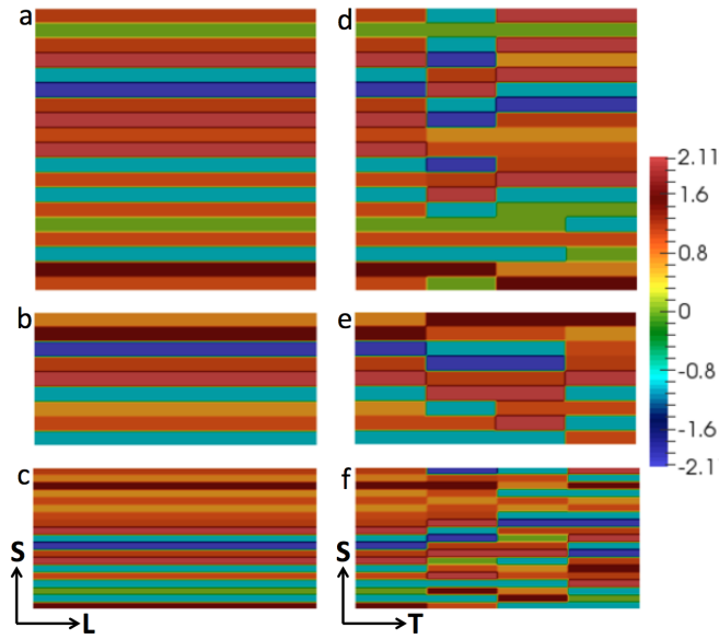
Figure 5: Different sheet microstructures used in the simulations Left: tension along L direction of a slab with (a) 19 grains of thickness 6 \mu m , (b) 9 grains of thickness 6 \mu m and (c) 19 grains of thickness 3 \mu m along the S direction. The rolling frame is shown at the bottom. Right: tension along T direction of a slab with (d) 19 grains of thickness 6 \mu m , (e) 9 grains of thickness 6 \mu m and (f) 19 grains of thickness 3 \mu m along the S direction. The rolling frame is shown at the bottom. The color-code is relative to the Euler angle \phi(rad) .
