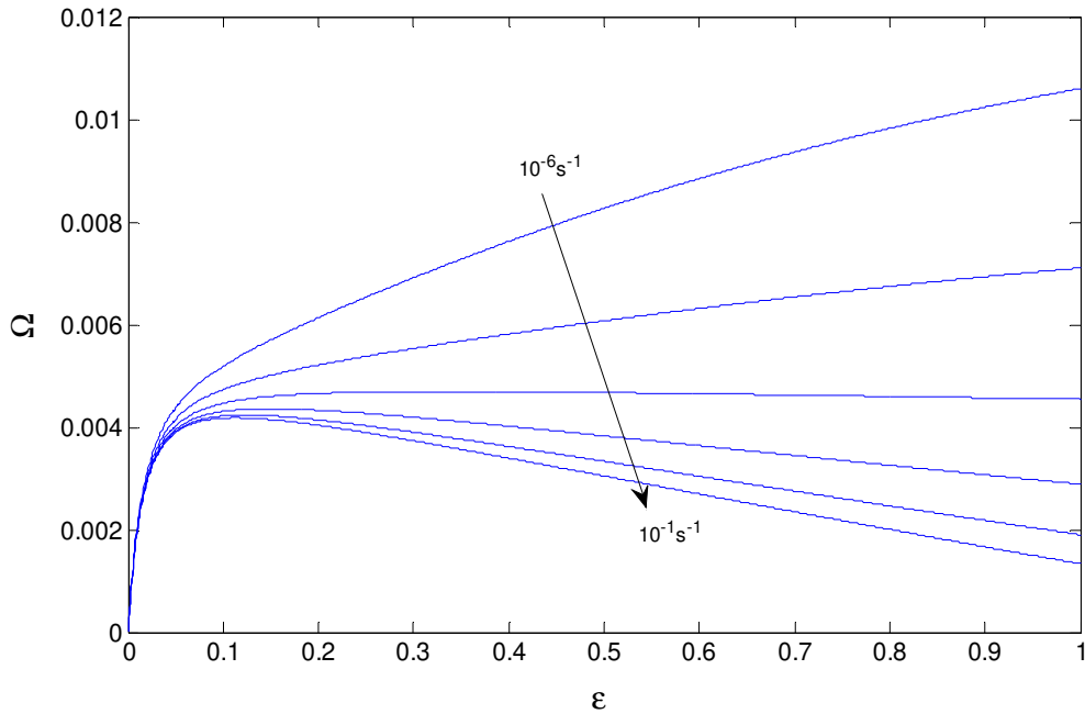
Fig.2. Strain dependence of the elementary strain \Omega at strain rates 10^{-6} , 10^{-5} , 10^{-4} , 10^{-3} , 10^{-2} and 10^{-1} s^{-1} .
