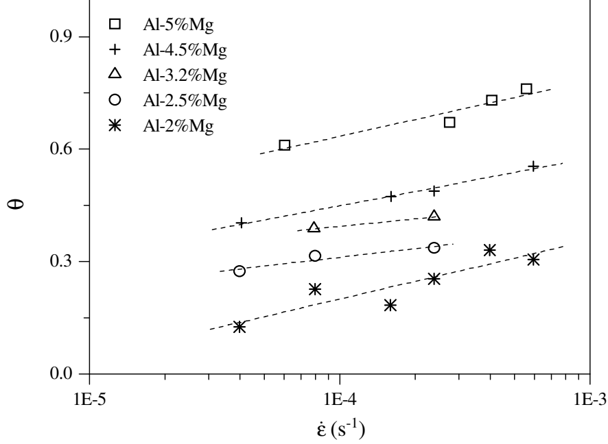
Fig. 3. Strain rate and Mg content dependences of the parameter \theta , comparison with Pink and Grinberg [14] results in the Al-5%Mg alloy.
