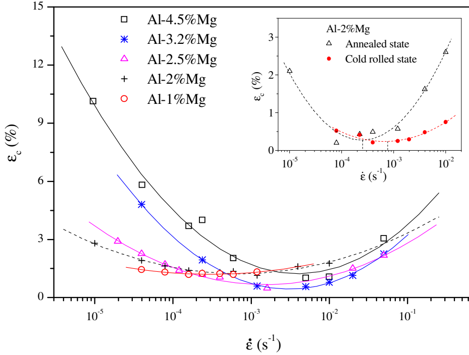
Fig. 5. Applied strain rate dependence of the critical plastic strain for different Al-Mg alloys. Inset: Effect of heat treatment (annealing at 400°C for 2h) on the critical strain in the Al-2%Mg, according to Ziani et al.[18].
