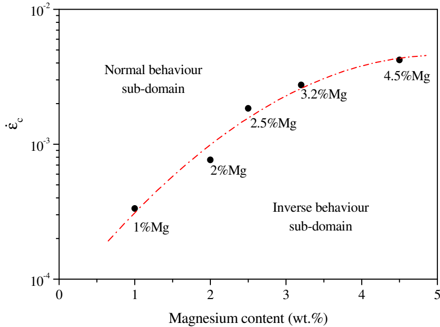
Fig. 6. Effect of the nominal concentration of Mg on \dot{\varepsilon}_c , the minimum of the curve \varepsilon_c(\dot{\varepsilon})
