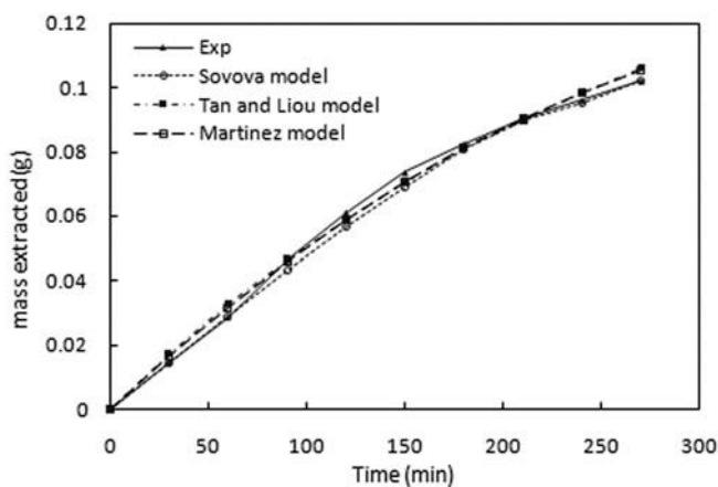
Figure 2. Comparison of experimental results and fitted OEC for SFE from rosemary leaves using the Sovova, Tan and Liou and Martínez models.
