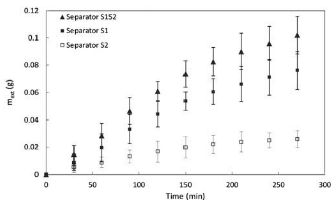
Figure 1. Kinetic SFE data from rosemary leaves at 180 bar and 50°C.
