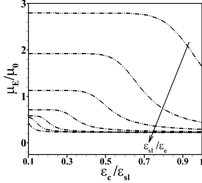
Figure 2. Dependence of scaled mobility ( \mu_E/\mu_0 ) of Sc-Ssl particles (Eq. 11) on the electrostatic softness of the core ( \epsilon_c/\epsilon_{sl} ) for various values of the shell electrostatic softness \epsilon_{sl}/\epsilon_e = 0.1, 0.15, 0.2, 0.3, 0.5, 0.7, 1 at fixed \lambda_{sl}^{-1} = 10 nm and \lambda_c^{-1} = 1 nm. Other model parameters: N_c = N_{sl} = 1 mM, z_c = z_{sl} = 1 , \kappa^{-1} = 1 nm, d = 10 nm, L = 100 nm. The direction of the arrow represents increasing values of \epsilon_{sl}/\epsilon_e .
