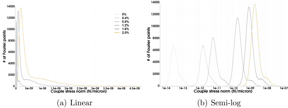
Figure 7: Couple stress norm \|\mathbf{M}\| histograms with (a) linear and (b) semi-logarithmic axes for the 20nm microstructure loaded from E_{22} = 0\% to 2% strain at \dot{E}_{22} = 1/s . Each histogram is computed using 256 bins, taking values from every Fourier point in the domain.
