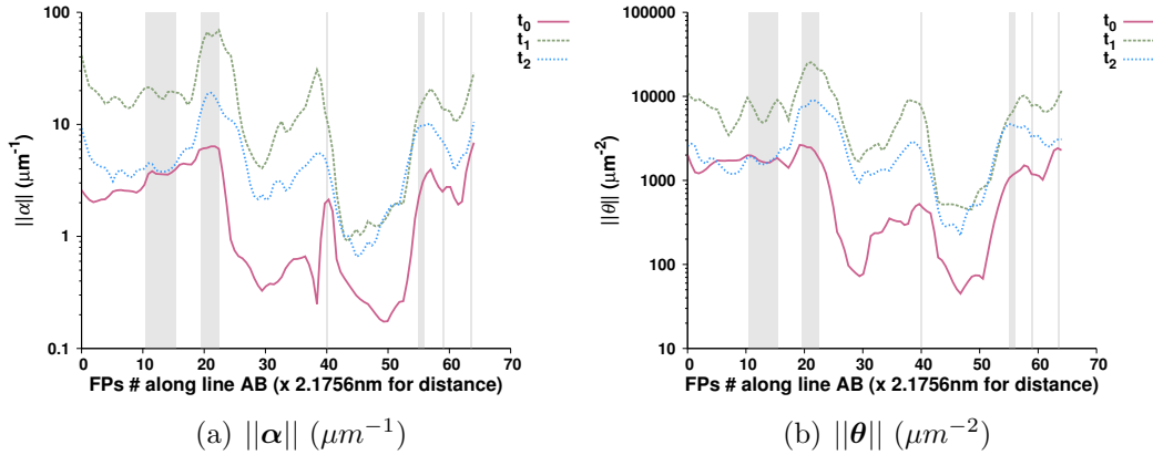
Figure 14: Log normal plot-over-line AB from figure 3 of (a) \|\alpha\| ( \mu\text{m}^{-1} ) and (b) \|\theta\| ( \mu\text{m}^{-2} ) for t_0 , t_1 and t_2 loaded to 2% strain at a rate of 1/s for the 20\text{nm} microstructure.
