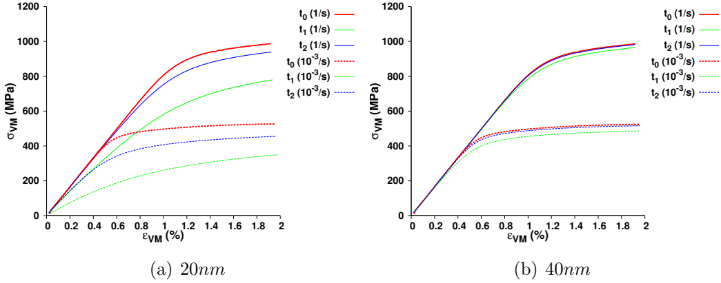
Figure 9: Comparison of VM Cauchy stress vs equivalent strain curves predicted for t_0 , t_1 and t_2 microstructures with average grain size (a) 20nm and (b) 40nm for strain rates \dot{E}_{22} = 0.001/s and \dot{E}_{22} = 1/s .
