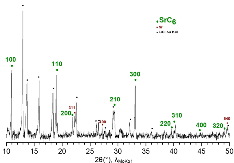
Fig. 3. hk0 X-ray diffraction pattern ( \lambda_{\text{MoK}\alpha 1} = 70.926 pm) of the first stage SrC 6 GIC ( I_C = 494 pm).
