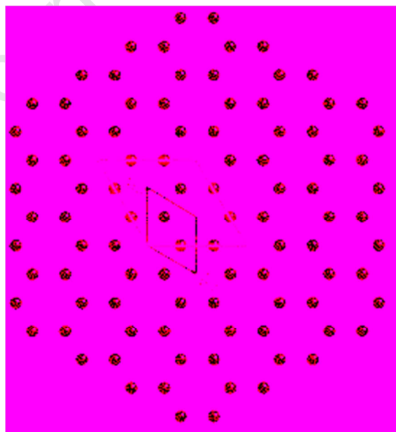
Fig. 4. 2D unit cells of graphene (____) and SrC 6 compound (____) rotated by 30^\circ .
