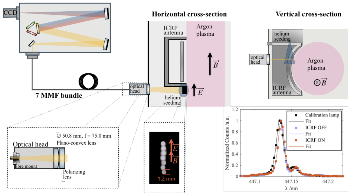
Figure 3: Set-up of the passive optical emission spectroscopy system and measured He I spectral line at 474.1 nm.
