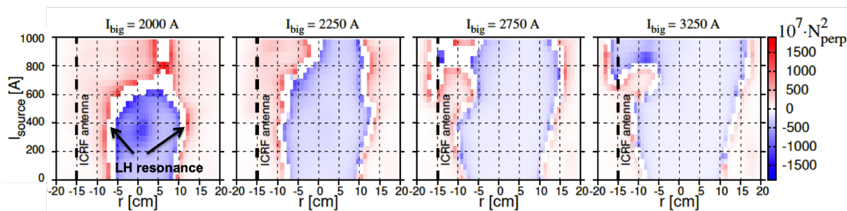
Figure 2: Perpendicular component of the refraction coefficients for the slow wave in a magnetised Ar plasma for k_{\parallel} = 10 \text{ m}^{-1} , a frequency of 6 MHz and typical IShTAR density profiles as presented in fig. 1.
