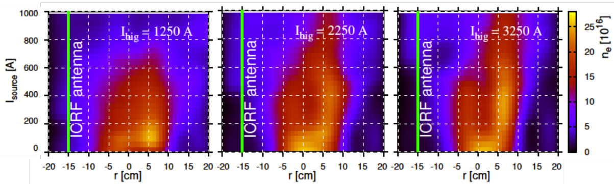
Figure 1: Radial plasma density profiles for various currents in the coils surrounding the main chamber ( I_{\text{big}} ) and plasma source ( I_{\text{source}} ). The radial position of the ICRF antenna is specified by a vertical green line.
