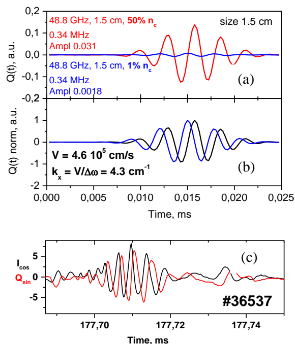
Figure 2. (a) Calculated Q(t) signals for linear (blue) and nonlinear (red) regimes; (b) normalized calculated signals; (c) I(t) and Q(t) DBS signals measured in Globus-M shot #36537, f=48 GHz.
