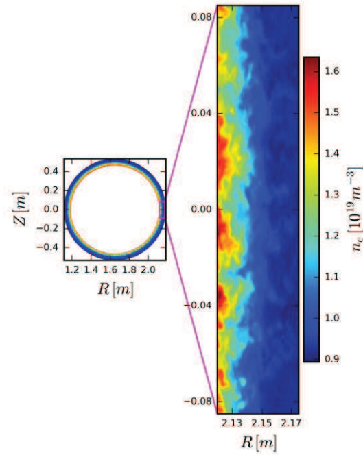
Fig. 1: GEMR electron density data on a poloidal plane cut, defined on a polar geometry, and zoom on region employed for REFMUL simulations.
