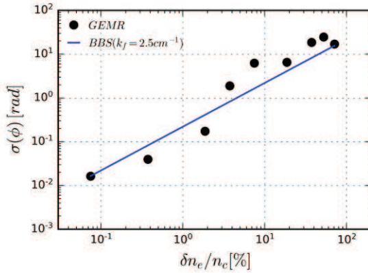
Fig. 2: Standard deviation of simulated reflectometry phase \phi(t) at the corresponding turbulence levels at the cut-off location \delta n_e/n_e . Also shown (solid line) is the theoretical estimate of 1D Bragg backscattering contributions.
