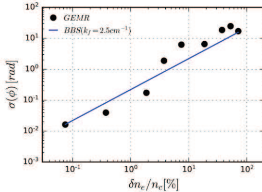
Fig. 2: Standard deviation of simulated reflectometry phase \phi(t) at the corresponding turbulence levels at the cut-off location \delta n_e/n_c . Also shown (solid line) is the theoretical estimate of 1D Bragg backscattering contributions.
