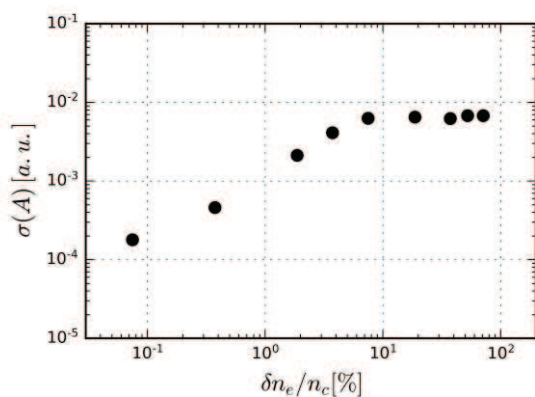
Fig. 3: Standard deviation of simulated reflectometry amplitude A(t) at the corresponding turbulence levels at the cut-off location \delta n_e/n_c .
