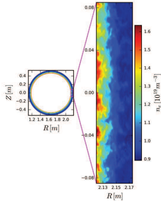
Fig. 1: GEMR electron density data on a poloidal plane cut, defined on a polar geometry, and zoom on region employed for REFMUL simulations.
