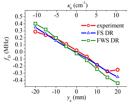
FIG. 4 Dependence of the DR signal frequency shift on the antenna vertical displacement y_a and fluctuation wavenumber. Circles – experiment; triangles – fast synthetic DR; squares full-wave synthetic DR.
