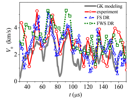
FIG. 6 Poloidal velocity temporal behavior. Thick line – computed directly by GK code, circles – measured; triangles – fast synthetic diagnostics; squares – full-wave synthetic diagnostics
