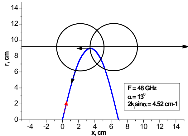
Figure 5. Ray tracing of the signal scattering off the filament 6cm.
