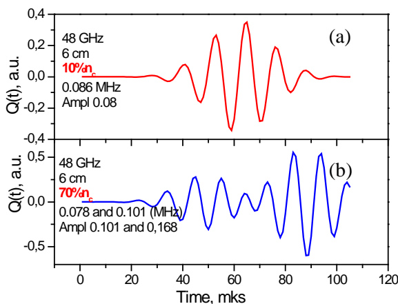
Figure 4. Calculated signal for 6cm filament diameter, 10% of critical density n c (a) and 70% of n c (b).
