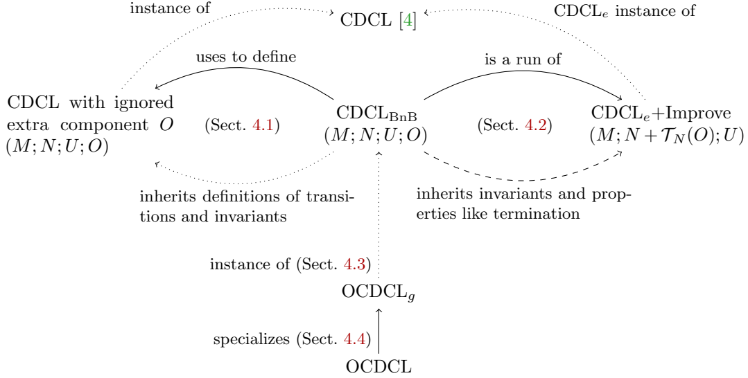
Figure 1: The calculi \text{CDCL}_{\text{BnB}} , \text{OCDCL} , and \text{CDCL}_e . Dotted links are locale instantiations and are for free, while dashed links indicate that some parts are for free.
