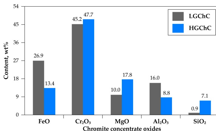
Figure 3. Chemical composition of the chromite concentrate samples.
