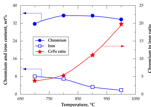
Figure 17. Evolution of chromium and iron content and chromium to iron ratio versus temperature during treatment of HGChC in a \text{Cl}_2 +air gaseous mixture.
