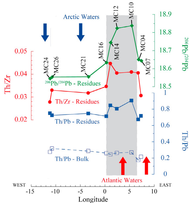
Figure 4. Th/Zr (red), Th/Pb (blue), and ^{206}\text{Pb}/^{204}\text{Pb} (green) ratios of surface sample detrital residues and Th/Pb ratios of bulk fractions. Sample sites follow the transect illustrated in Figure 1 and their geochemical and isotopic compositions display a spatial zonation in the Strait. Arrows illustrate the main active currents.
