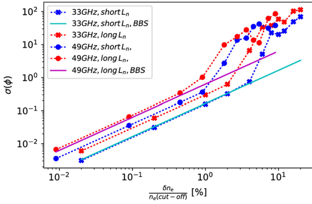
FIG. 11. Standard deviation of reflectometry \varphi(t) signals for turbulence level scans with 2 probing frequencies f_p and 2 density gradient scale lengths L_n , for outward radial plasma flows. Theoretical values estimated from Eq. (1) for two of the simulated cases are also shown in solid lines.
