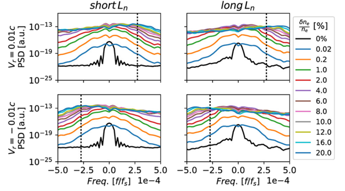
FIG. 9. Power spectra of reflectometry complex amplitude signals A(t)e^{i\varphi(t)} for turbulence level scans in both inward and outward radial plasma flow directions, with f_p = 33 GHz probing frequency, and two different density gradient lengths L_n of background slab plasmas.
