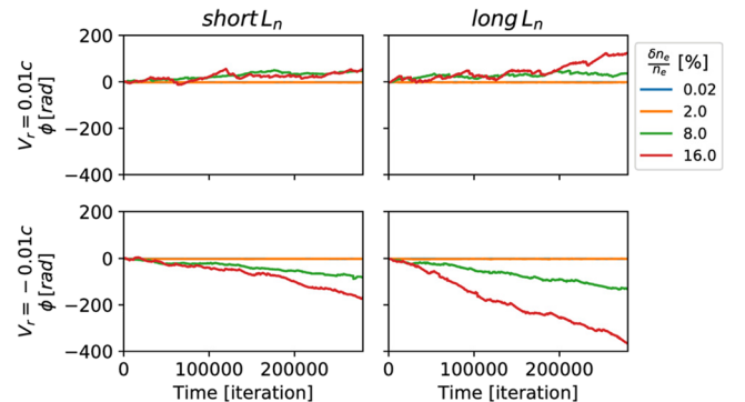
FIG. 10. Time traces of reflectometry \varphi(t) signals for turbulence level scans with f_p = 33 GHz probing frequency and 2 density gradient scales L_n for both cases of inward and outward radial plasma flow.
