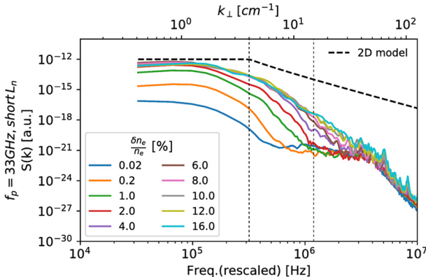
FIG. 4. Power spectra of A(t)e^{i\varphi(t)} signals on the re-scaled single-sided frequency axis and corresponding k_{\perp} -axis, for a turbulence level scan with probing frequency f_p = 33 GHz and short density gradient scale length L_n .
