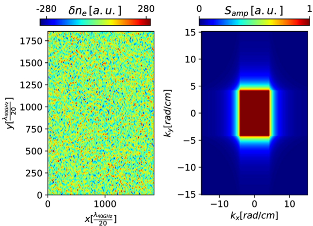
FIG. 1. Example of a 2D density turbulence realization (left) generated with a Kolmogorov-like model of a given amplitude k -spectrum (right).
