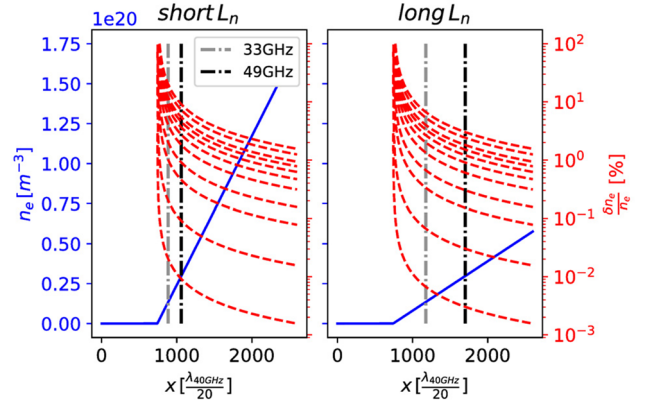
FIG. 2. Linear background density profiles (solid blue) and radial positions of the f_p = 33 GHz and f_p = 49 GHz cutoffs, together with the set of density turbulence level profiles (dashed red) employed for the numerical plasmas.
