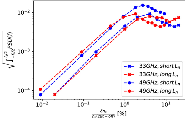
FIG. 6. Root mean square (total integrated power spectra) of A(t)e^{i\varphi(t)} signals for turbulence level scans with 2 probing frequencies f_p and 2 density gradient scale lengths L_n .
