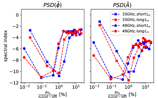
FIG. 5. Spectral index obtained from the fluctuating components of A(t) and \varphi(t) signals in turbulence level scans with 2 probing frequencies f_p and 2 density gradient scale lengths L_n .
