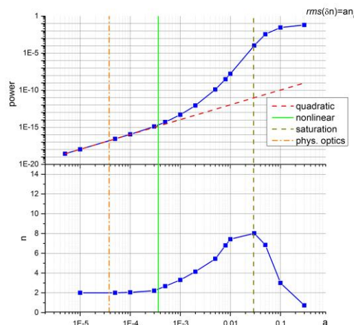
Fig 1. Calculation results for f=30\text{GHz} , L=20\text{cm} , l_{cx}=1.3\text{ cm} , l_{cy}=1.3. \text{cm} , \vartheta=40^\circ . Fig 2. Calculation results for f=30\text{GHz} , L=20\text{cm} , l_{cx}=1.7\text{ cm} , l_{cy}=1.7. \text{cm} , \vartheta=30^\circ .
