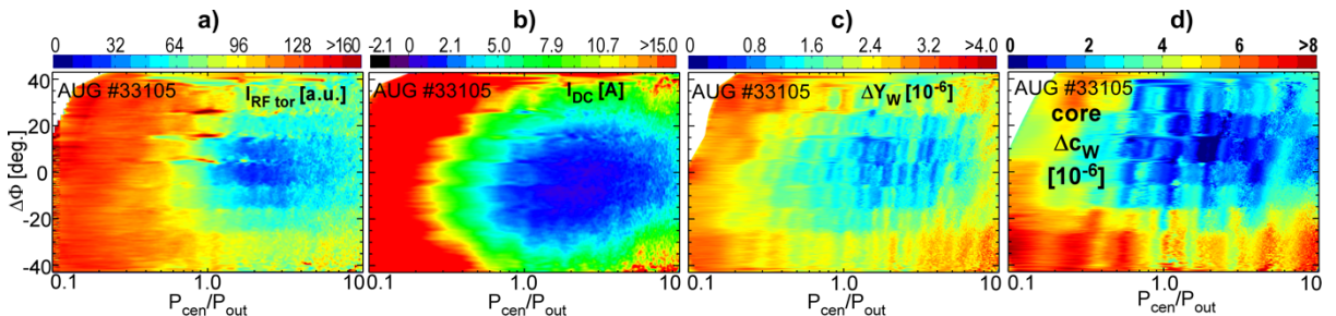
FIG. 1. RF feeding diagrams using the strap power balance P_{cen}/P_{out} and phase deviation from dipole \Delta\Phi as variables in a discharge with P_{ICRF}=1MW ; local measurements at a single antenna limiter tile of (a) the toroidal RF current, (b) the DC current circulation and (c) of the increment of the W sputtering yield; (d) increment of the W content in plasma at T_e \approx 1.5 keV.
