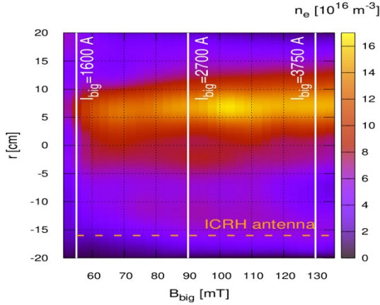
FIG. 5. Radial profile of the plasma density in the main vacuum vessel as a function of the magnetic field in the center of the main vessel. The range of magnetic fields B_{big} corresponds to the change of current in the set of big coils I_{big} in Fig. 4. (a)-(c).
