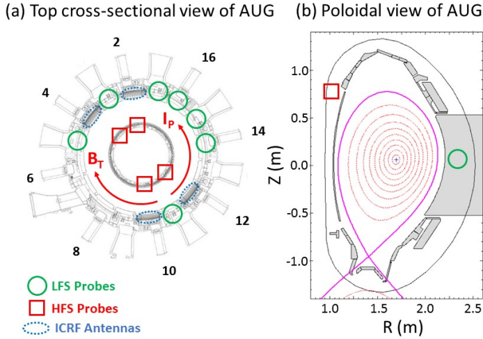
FIG. 3: (a) top and (b) poloidal cross-sectional views of the AUG. The positions of the low-field side (LFS) and the high-field side (HFS) B-dot probes is shown. The HFS probes are positioned radially opposite to the ICRF antennas.
