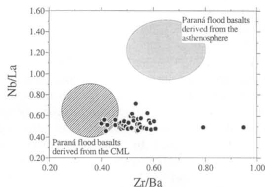
Fig. 3. Nb/La vs. Zr/Ba for Ferrar lavas from Victoria Land. Fields taken from [33].
