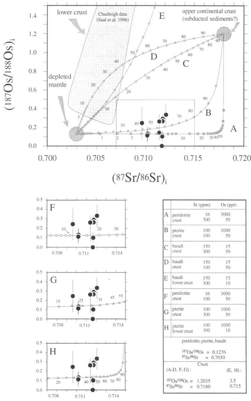
Fig. 5. Initial ^{187}\text{Os}/^{188}\text{Os} vs. initial ^{87}\text{Sr}/^{86}\text{Sr} . Model curves represent mixing between mantle peridotite and crustal sediments (source contamination) and mantle magmas (basalts and picrites) and crust (crustal contamination). The crustal end-member was chosen to be variable in Sr content (100–300 ppm). The ^{187}\text{Os}/^{188}\text{Os} – ^{87}\text{Sr}/^{86}\text{Sr} reference data field for lower crustal xenoliths from the Chudleigh province in NE Australia was kindly made available by Alberto Saal ([51] and Saal et al. unpubl. data).
