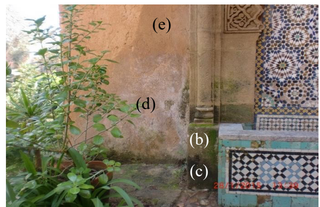
Fig. 2 – Walls bases in calcarenite in the garden of Udayas already restored; soil water rises by capillary transfer in the base, contour scaling initiated on the part in contact with the ground in zone (a) where evaporation is faster than capillary rise, development of green algae (zone b) and lichen (zone c), white efflorescence of salts (zone d) where the water evaporates on the surface, (zone e) always wet.
