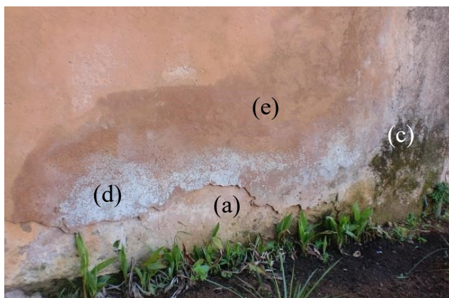
Fig. 2 – Walls bases in calcarenite in the garden of Udayas already restored; soil water rises by capillary transfer in the base, contour scaling initiated on the part in contact with the ground in zone (a) where evaporation is faster than capillary rise, development of green algae (zone b) and lichen (zone c), white efflorescence of salts (zone d) where the water evaporates on the surface, (zone e) always wet.
