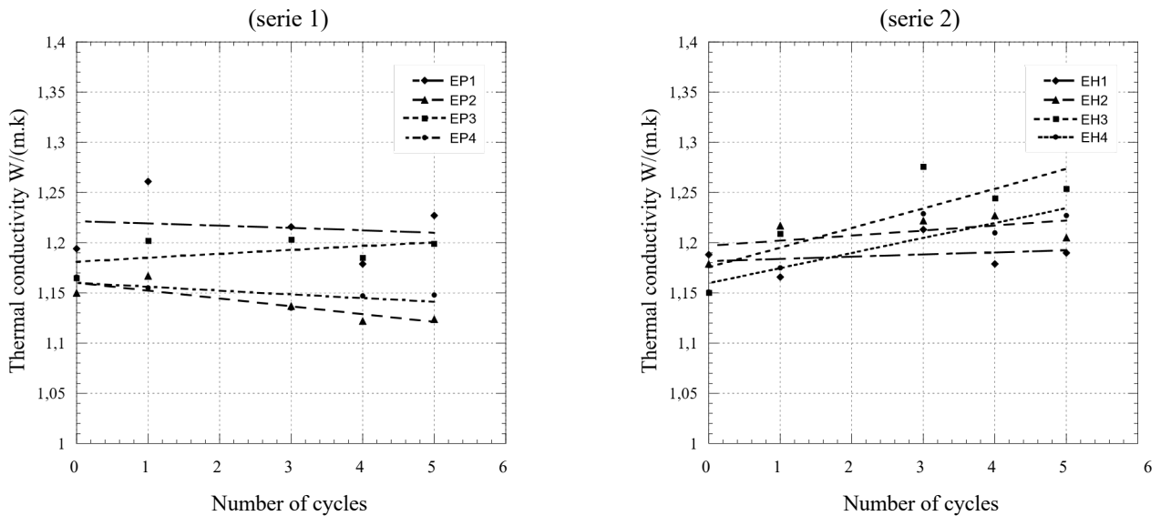
Fig. 6 - Evolution of average thermal conductivity for calcarenite samples (series 1 and 2) during salt weathering cycles by imbibition-drying.
