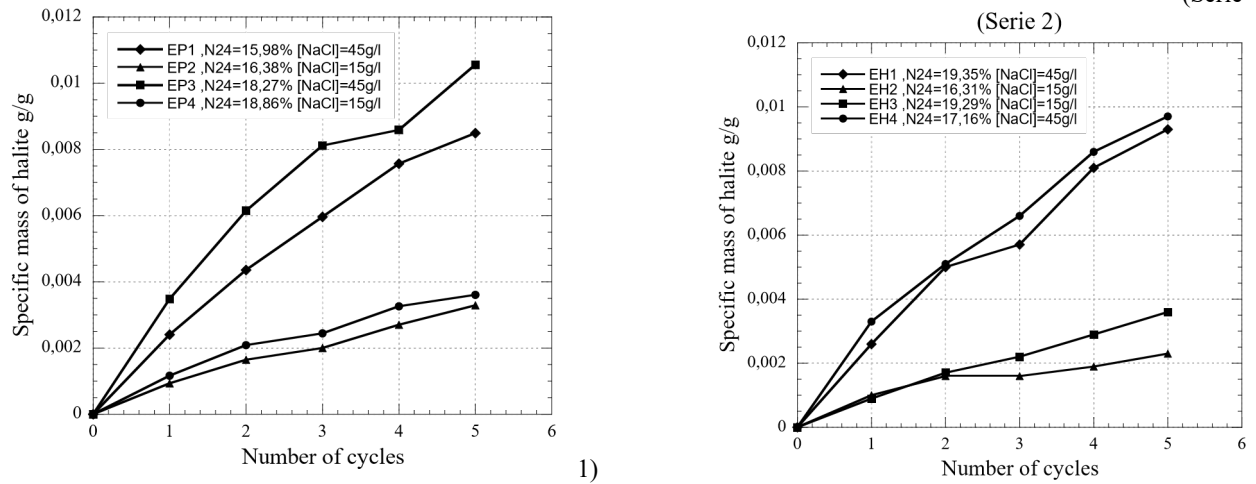
Fig. 4 – Evolution of specific mass of precipitated halite during crystallization-dissolution cycles.
