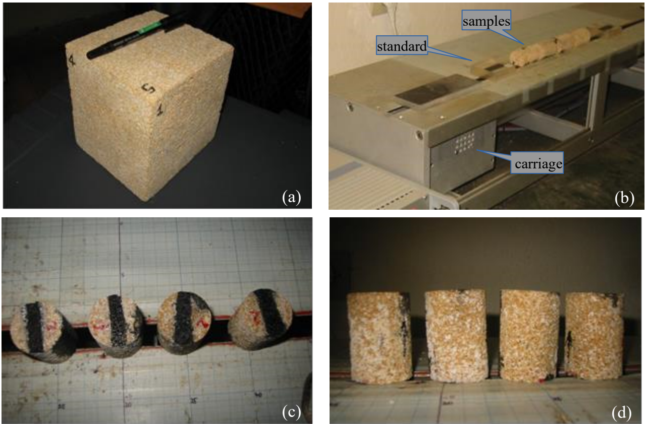
Fig. 3 – (a) Calcarenite block used for coring eight identical cylindrical samples: (c) four cores taken parallelly to the sediment bedding (series 1) and (d) four other perpendicularly to this one (series 2). (b) Four calcarenite cores between two standard samples positioned along the scanning direction on the platform of thermal conductivity scanner (TCS). The pictures (c) and (d) are taken after the first dissolution-crystallization cycle, and show the NaCl efflorescence formation.
