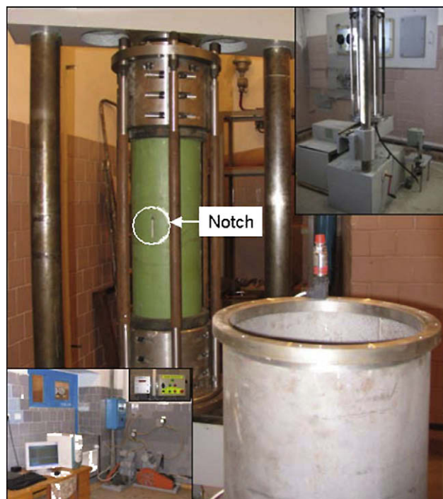
Fig. 3 – General view of designed testing equipment (protective housing is removed).
