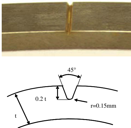
Fig. 13 – Notch geometry.
