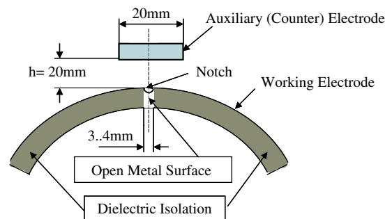
Fig. 14 – Mutual location of working electrode (specimen) and auxiliary (counter) electrode.
