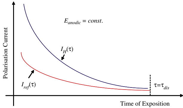
Fig. 15 – Schematic view of hydrogen discharging process under anodic polarisation.
