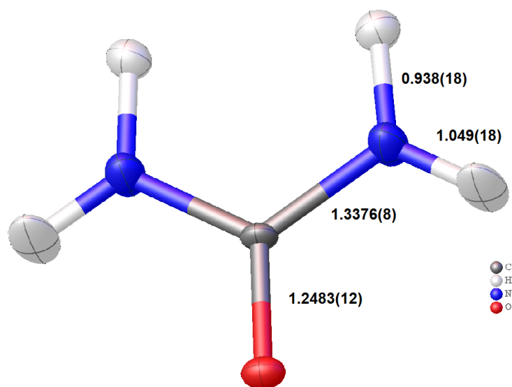
Fig. 11: Hirshfeld atom refined structure of urea based on powder diffraction data with refined bond distances in Å and anisotropic displacement parameters at the 50% probability level (half of the molecule is symmetry-independent); courtesy of B. Svane and B. B. Iversen, Aarhus University.
