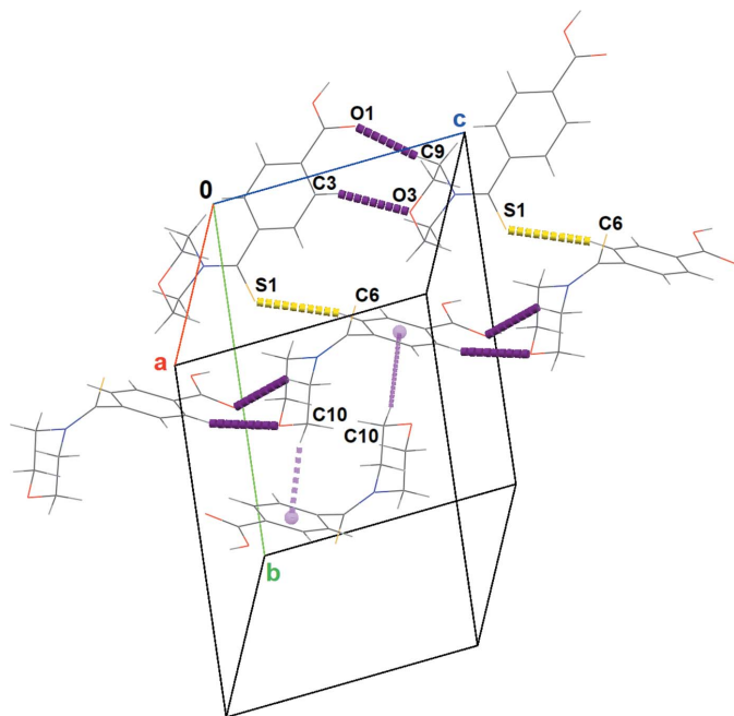
Figure 4 A projection of the three-dimensional network of intermolecular interactions (purple and yellow dotted lines) of the title compound. The C—H... \pi interactions are shown with violet dashed lines.
