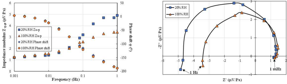
Figure 7: Comparison of EPIS measurements: (a) Bode plot, and (b) Nyquist plot at different humidification conditions at 0.8 A.cm -2 . (Solids lines are only for illustration)
