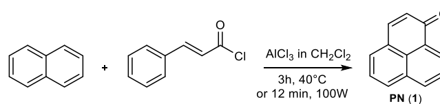
Scheme 1. Phenalenone Synthesis
