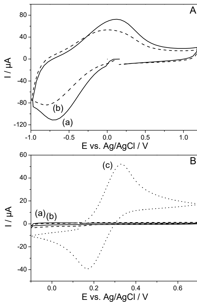
Fig. 3. (A) Cyclic voltammograms recorded at 5 \text{ V s}^{-1} in 0.1 \text{ M NaNO}_3 solution using a mesoporous silica film bearing \text{Fe(Htrz)}_3 (a) after or (b) before treatment in an ethanol solution containing 0.1 \text{ M HCl} for 15 \text{ min} . (B) Cyclic voltammograms recorded at 100 \text{ mV s}^{-1} in 1 \text{ mM Fc(MeOH)}_2 ( +0.1 \text{ M NaNO}_3 ) aqueous solution using the same electrode as in (A), also (a) after or (b) before treatment in \text{HCl/ethanol} ; the dotted line (c) is the voltammogram recorded at bare ITO electrode.
