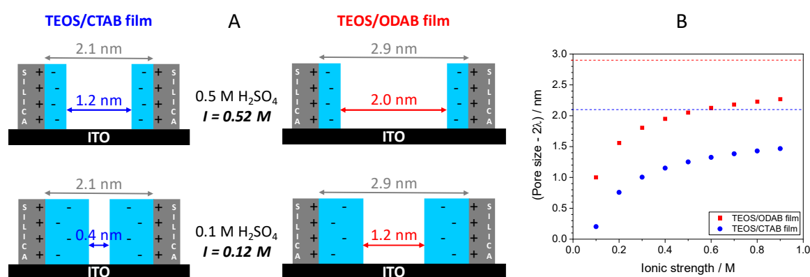
Figure 5. (A) Schematic view of mesopore channels of CTAB- and ODAB-based films with electrical double layers corresponding to pH 0.3 and 1.0. (B) Variation of the effective pore diameters (i.e., “pore size – 2\lambda ” values) of both films as a function of the ionic strength (dashed lines represent the pore diameter of both mesoporous films).
