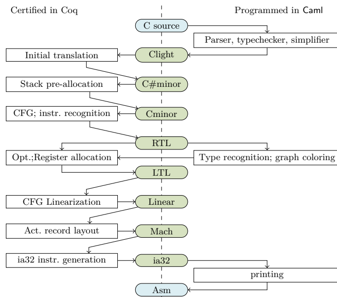
Fig. 1. CompCert architecture.
