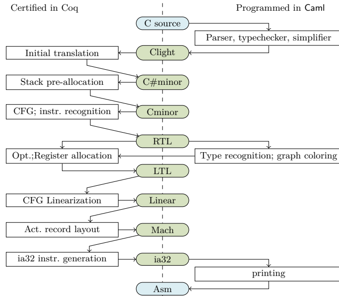
Fig. 1. CompCert architecture.
