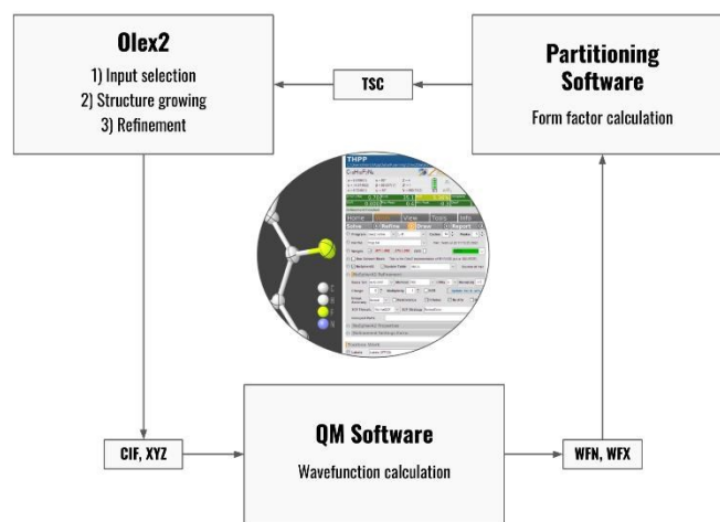
Figure 2. Flowchart of the process behind HAR controlled by NoSpherA2 and a visual representation of the GUI for NoSpherA2 inside Olex2 .
