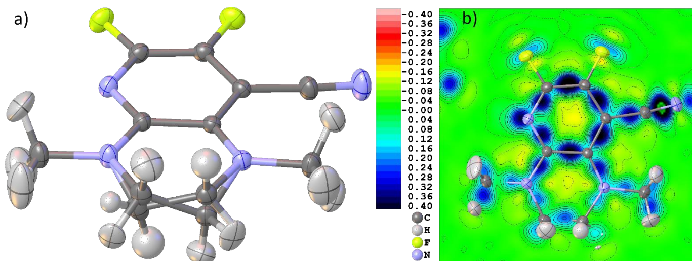
Figure 5. a) Final HAR geometry after disorder treatment of THPP. b) Dynamic deformation density distribution in the main molecular plane of the molecule. Color scale legend in eÅ -3 . Atomic anisotropic and isotropic displacement parameters at 80% probability level.
