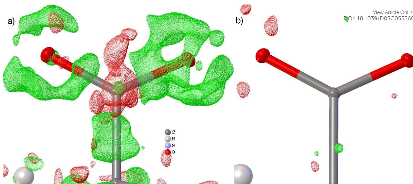
Figure 3. Visualization of the residual density distribution of the carboxylate group in L-Ala after IAM (a) and HAR, model vi (b). The residual density was calculated with Olex2 from fcf files and plotted on a grid of 0.05 Å with an iso-value of 0.10 eÅ -3 (green = positive, red = negative). In the IAM plot, residual density regions of a different functional group that obstructed the view onto the carboxylate were manually removed.
