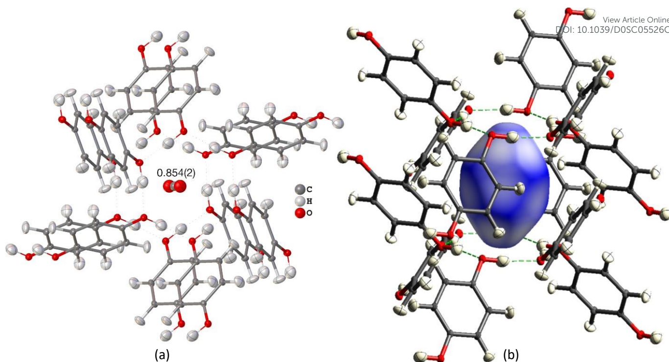
Figure 4. HAR-refined hydroquinone-CO 2 clathrate structure (HQ-CO 2 ) with anisotropic displacement parameters depicted at 80% probability level. The cluster of the guest CO 2 molecule with the 12 surrounding HQ molecules encapsulating CO 2 inside a void is shown as used in the wavefunction calculation underlying the non-spherical form factor generation. (a) Final refined geometry and partial occupation number of CO 2 . (b) Hirshfeld surface representation of CO 2 inside the void mapped with the property d_{\text{norm}} . Color scale from 0.08 (white) to 0.77 (blue). Generated with CrystalExplorer 87 .
