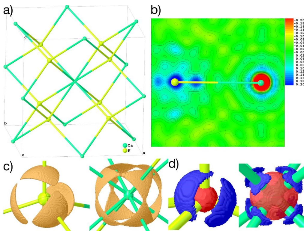
Figure 6. a) Structure of the explicit cluster used for the calculation of the wavefunction of CaF 2 during HAR, coinciding with a unit cell. (b) 2D-plane of dynamic deformation density, color scale in steps of 0.02 eÅ -3 . (c) 3D-isosurfaces of the ELI-D with iso-values of 1.835 (F) and 1.910 (Ca). (d) 3D-isosurfaces of the atomic deformation Hirshfeld densities at isovalues of ± 0.411 (F) and ± 0.088 (Ca) eÅ -3 . All maps are calculated on a 0.01 Å grid and plotted using Olex2 . Displacement parameters at 80% probability level.
