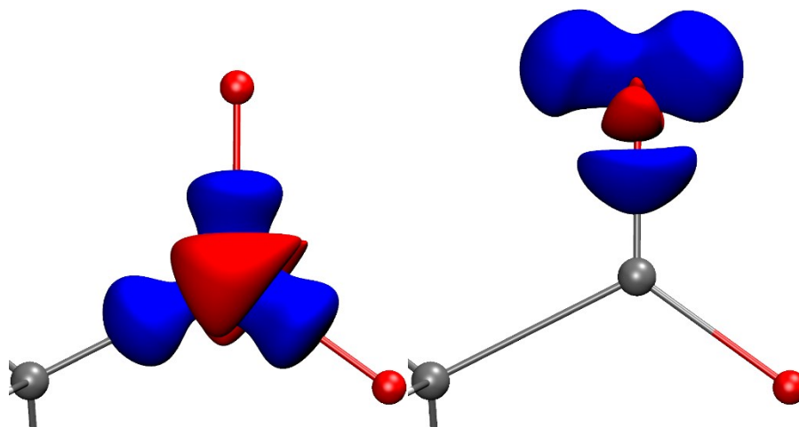
Figure 1. Deformation Hirshfeld densities 12 for the carbon (left) and oxygen (right) atoms in the carboxylate group of Gly-L-Ala, i.e. difference between the spherical atomic electron density used in the IAM and the non-spherical Hirshfeld atom density used in HAR (IAM minus HAR). Red = negative, blue = positive. Isovalue = 0.17 eÅ -3 .
