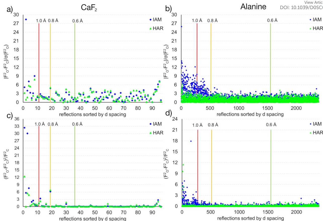
Figure 7. Differences of observed and calculated structure factors versus resolution for \text{CaF}_2 and L -Ala for the IAM and the HAR models.
