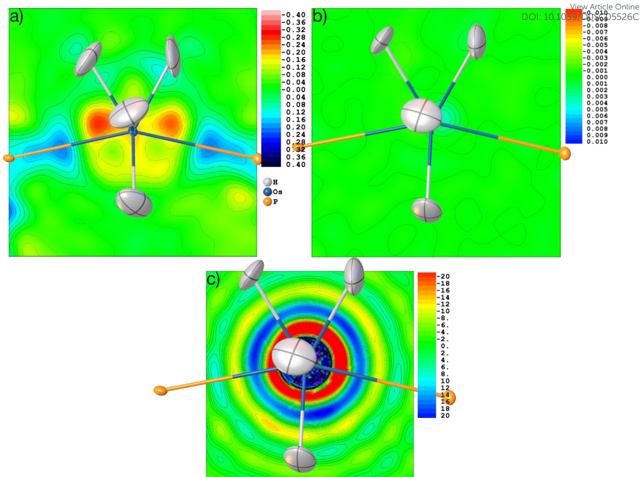
Figure 10. Residual electron density after refinement against theoretical structure factors in a) IAM model and b) HAR model. c) Electron density as the Fourier transform of the theoretical structure factors in the vicinity of the Os atom, showing Fourier truncation ripples. Three different contour intervals (see text). Color scale in \text{e}\text{\AA}^{-3} . Displacement parameters at 80% probability level.
