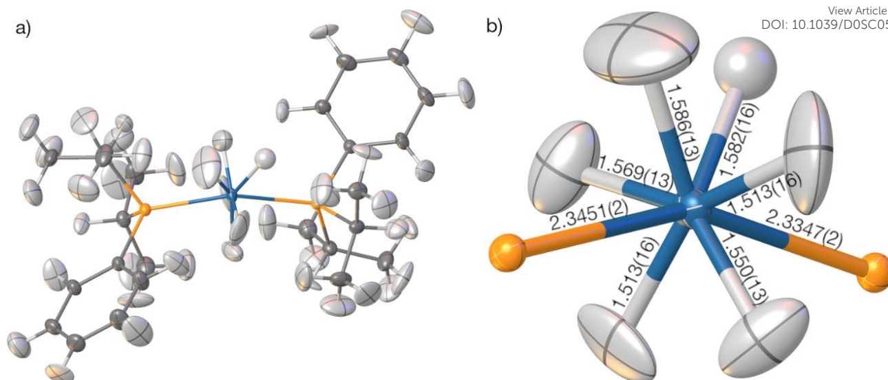
Figure 9. a) HAR-refined molecular structure of \text{OsH}_6(\text{PC}_{12}\text{H}_{19})_2 with the DKH2-PBE/x2c-TZVPP model at full resolution. (b) Coordination geometry of the Os atom with the freely refined distances to the six nearest hydrogen and two nearest phosphorus atoms. All displacement parameters are displayed at 80% probability level.
