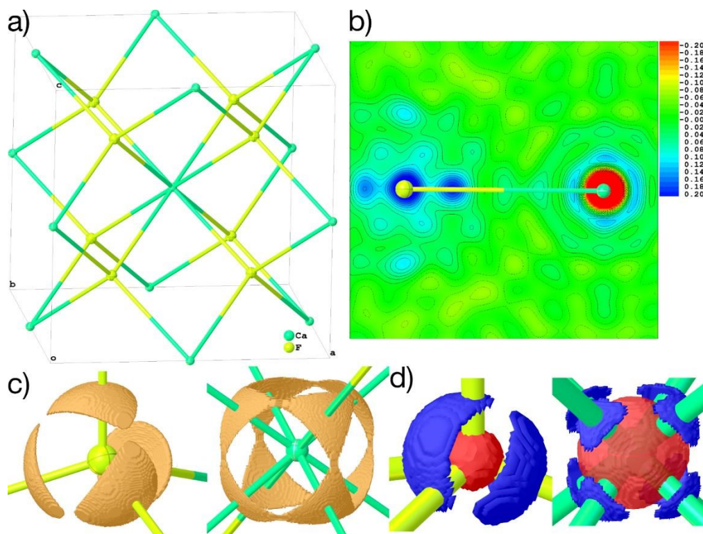
Figure 6. a) Structure of the explicit cluster used for the calculation of the wavefunction of CaF 2 during HAR, coinciding with a unit cell. (b) 2D-plane of dynamic deformation density, color scale in steps of 0.02 eÅ -3 . (c) 3D-isosurfaces of the ELI-D with iso-values of 1.835 (F) and 1.910 (Ca). (d) 3D-isosurfaces of the atomic deformation Hirshfeld densities at isovalues of ± 0.411 (F) and ±0.088 (Ca) eÅ -3 . All maps are calculated on a 0.01 Å grid and plotted using Olex2 . Displacement parameters at 80% probability level.
