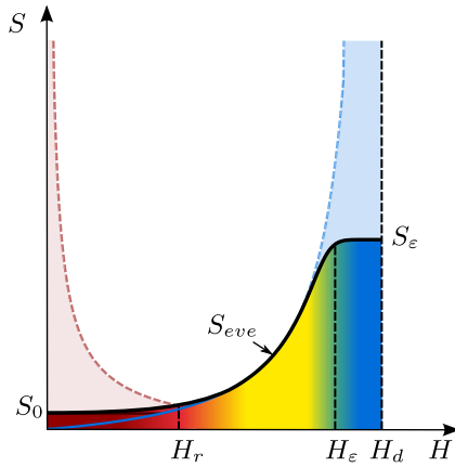
FIG. 4. Proposed characteristic dependence of the relaxation size S_{\text{eve}} with magnetic field. S_{\text{eve}} has two contributions: S_{\text{opt}} and S_{\text{rel}} (see Fig. 3). S_{\text{eve}} goes to a constant value S_0 at low fields. This is a good approximation since at low fields ( H < H_r ) the domain wall velocity is dominated by the exponential time scale and at higher fields ( H > H_r ) it is dominated by S_{\text{rel}} . A saturation of S_{\text{rel}} is considered in order to arrest the divergence of the domain wall velocity near the depinning field. For H < H_\varepsilon , S_{\text{rel}} is barely changed, but for H > H_\varepsilon a saturation to S_\varepsilon is reached.
