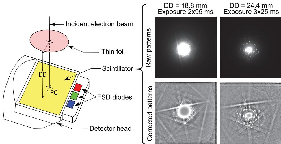
Fig. 1. (left) Scheme of the “on-axis” TKD detector head which includes a forescatter electron detector (FSD) and a scintillator. The projection geometry is defined by the sample-to-detector distance (DD) and the position of the pattern centre (PC). (right) EDP before and after background correction. Both patterns are acquired approximately at the same location using the two sets of acquisition parameters summed up in Table 1. (For interpretation of the references to colour in this figure legend, the reader is referred to the web version of this article.)
