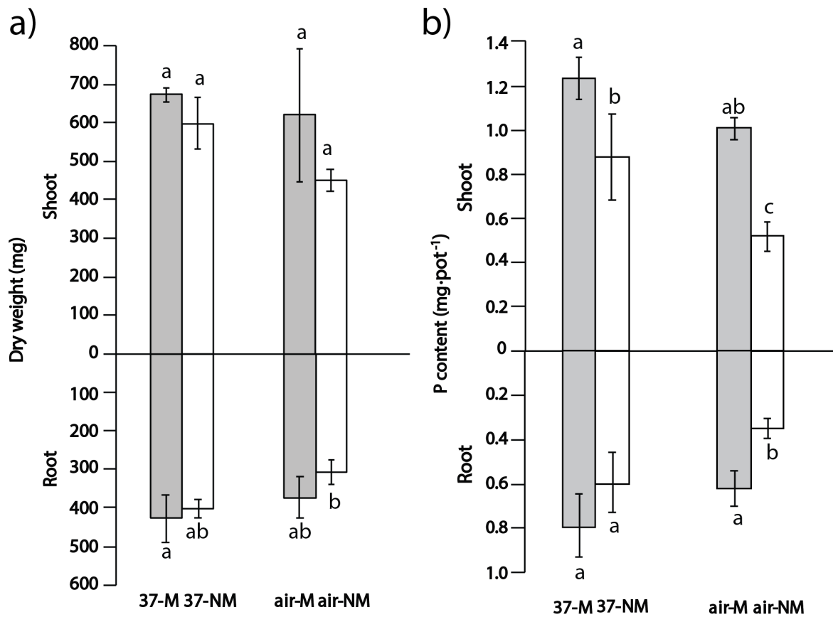
Fig. 3 a) Alfalfa shoot dry weight (total per pot) and b) P content of alfalfa shoots in compartment devices with 37 \mu\text{m} (37) or 37-1000-37 \mu\text{m} (air) mesh with (M) and without (NM) arbuscular mycorrhizal inoculation. Means followed by the same letter do not differ significantly using two-way ANOVA and Tukey (HSD) post-hoc tests ( P < 0.05 )
