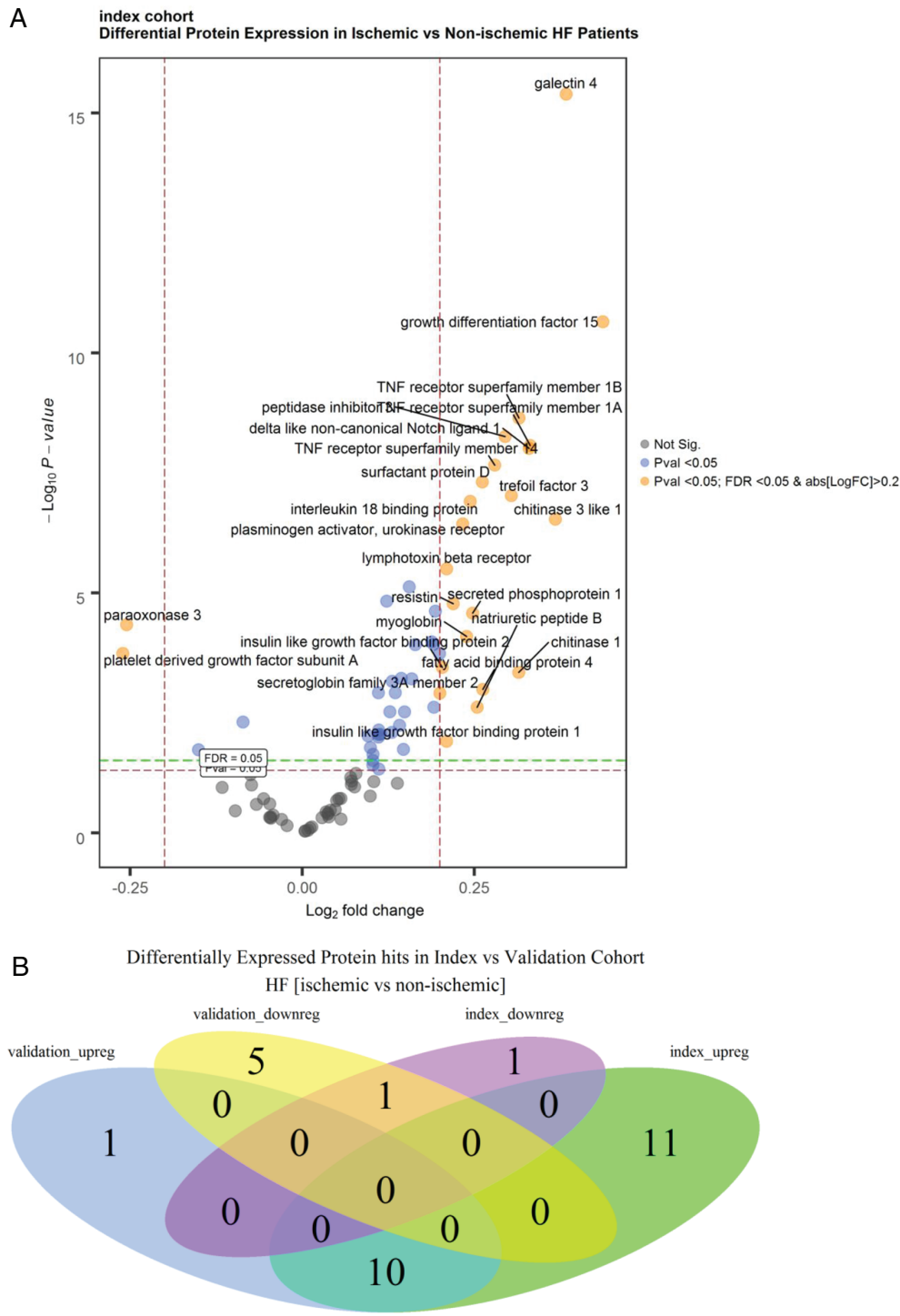
Figure 2 Differential protein expression in ischaemic relative to non-ischaemic heart failure (HF) patients. (A) Volcano plot of differential protein expression (y-axis significance, x-axis effect size (positive = up-regulated, negative = down-regulated; labelled = significant differentially expressed proteins). (B) Venn diagram of number of significantly differentially expressed proteins in index cohort (main) and validation cohort. Consistently, no proteins were up-regulated in one cohort but down-regulated in the other, nor vice versa. FC, fold change; FDR, false discovery rate; TNF, tumour necrosis factor.
