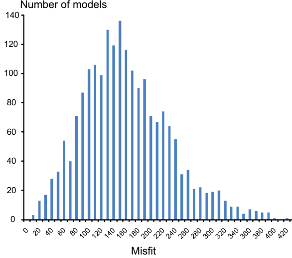
Figure 4: Mifsit repartition computed from equation 4. Only the 100 selected models are used as seeds to generate Markov chain of models and four of them have a misfit below 10 thus are considered as posterior models.
