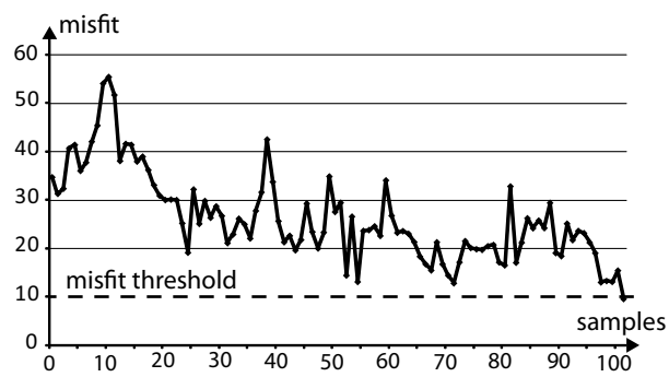
Figure 8: Misfit evolution for one seed model. The Markov chain stops when the misfit is below the input threshold and the last sample is used to compute posterior statistics.
