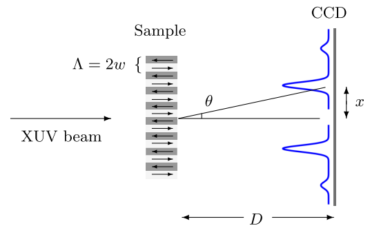
FIG. 9. Simplified sketch of the scattering geometry illustrating the link between scattering peak locations on the CCD and the periodicity of the magnetic domains.
