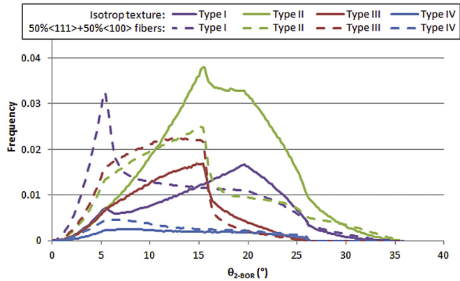
Fig. 10. Frequency of special GB types as a function of \theta_{2-BOR} deviation for two textures (isotropic and fiber like).
