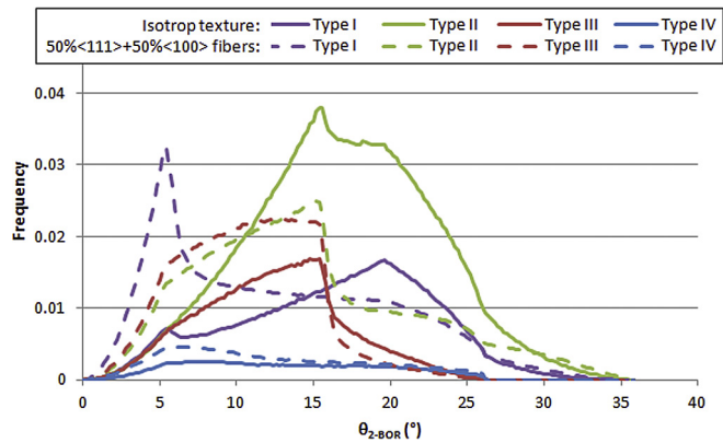
Fig. 10. Frequency of special GB types as a function of \theta_{2\text{-BOR}} deviation for two textures (isotropic and fiber like).
