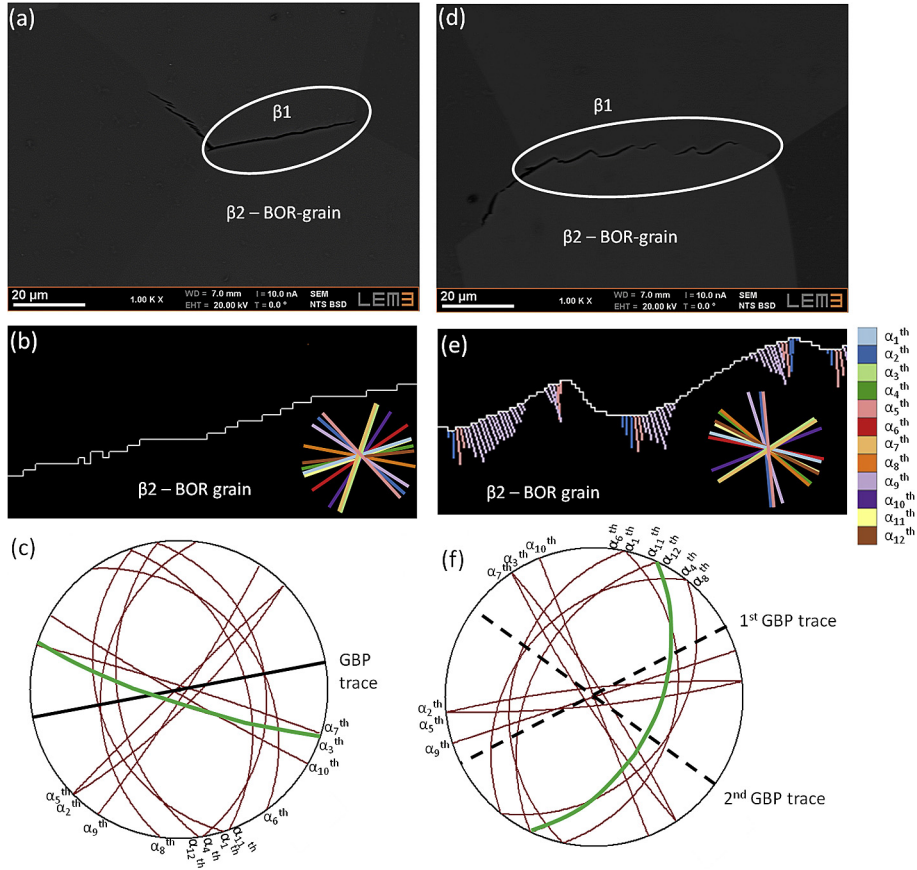
Fig. 8. Example A (planar GB) and B (zig-zag GB) showing the inconsistency between the observation and the predicted HP variants: (a,d) BSD image showing the \beta/\alpha/\beta interface and the BOR grain, (b,e) the predicted HP variants along the GB, and (c,f) the 12 HPP and the GBP trace projected on a pole figure, the HP of the observed variant is colored in green. (For interpretation of the references to colour in this figure legend, the reader is referred to the web version of this article).
