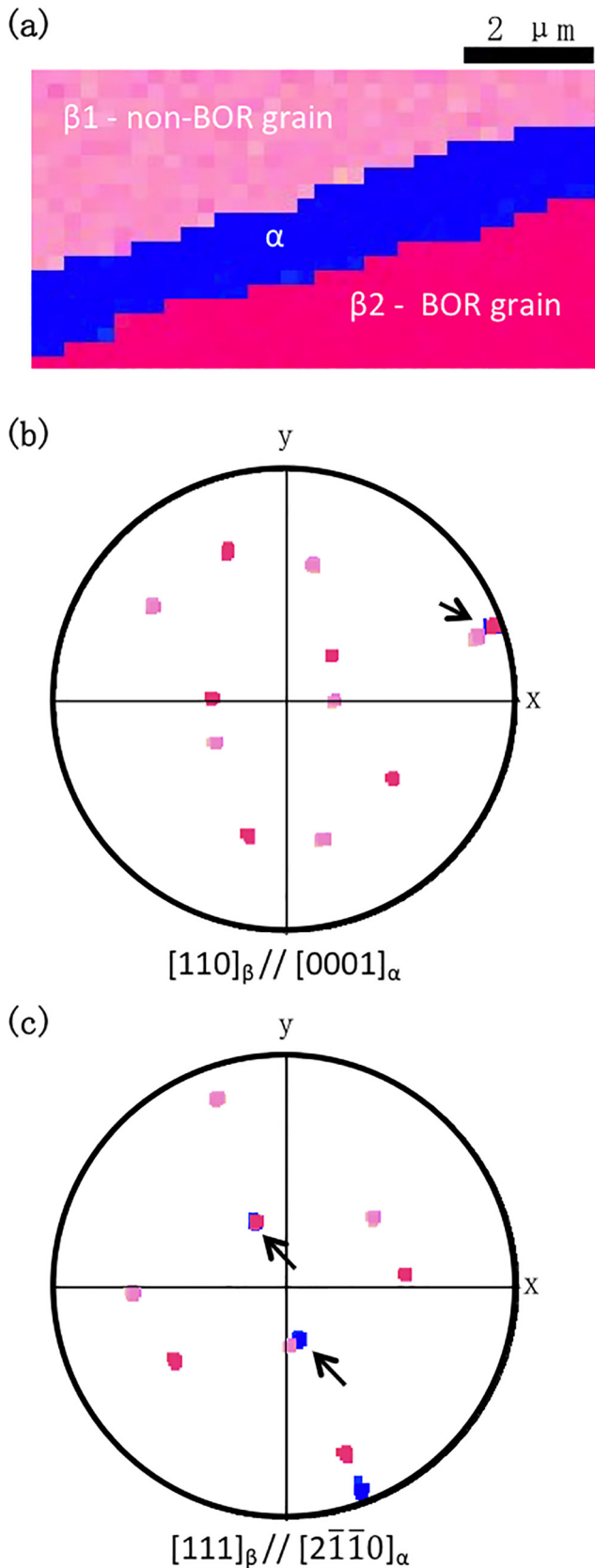
Fig. 6. A transformed GB satisfying the double-BOR criteria (with a deviation of 5.9^\circ ): (a) EBSD map showing \beta_1 and \beta_2 grains colored in light and dark pink and \alpha_{GB} layer in blue (The BOR grain and non-BOR grain are indicated); (b) Superimposed [110]_{\beta_1/\beta_2} and [0001]_{\alpha_{GB}} pole projections (the arrow indicates the 3 overlapping poles according to the double-BOR criterion); (c) Superimposed \langle 111 \rangle_{\beta_1/\beta_2} and \langle 2\bar{1}\bar{1}0 \rangle_{\alpha_{GB}} pole
