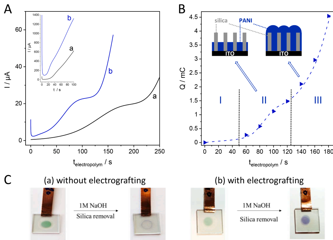
Fig. 2. (A) I - t curves PANI electropolymerization (0.1 M aniline in 0.5 M \text{H}_2\text{SO}_4 , E_{\text{app}} = +0.85 V) at ITO electrodes covered with a mesoporous silica film without (a) and with (b) electrografting of aminophenyl groups; inset: I - t curves in the absence of silica membrane on ITO. (B) Variation of charge ( Q ) measured as a function of electropolymerization time, integrated from I - t curves obtained in the same conditions as (A); inset: schematic view of PANI growth inside and outside the mesoporous film (stages II and III of electropolymerization). (C) Photographs of PANI on ITO/mesoporous silica film, before and after etching in 1 M NaOH, for sample prepared without (a) and with (b) electrografting.
